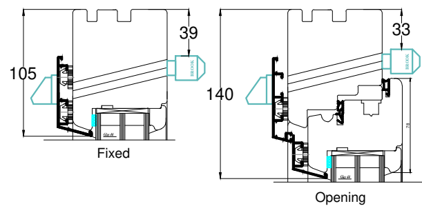
Trickle vents in 20mm thickened frame head
