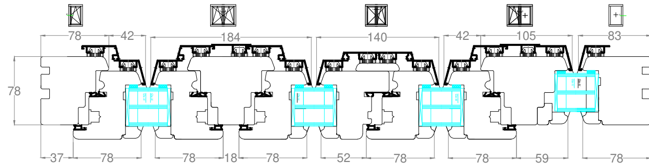
Trickle vents in 20mm thickened frame head
